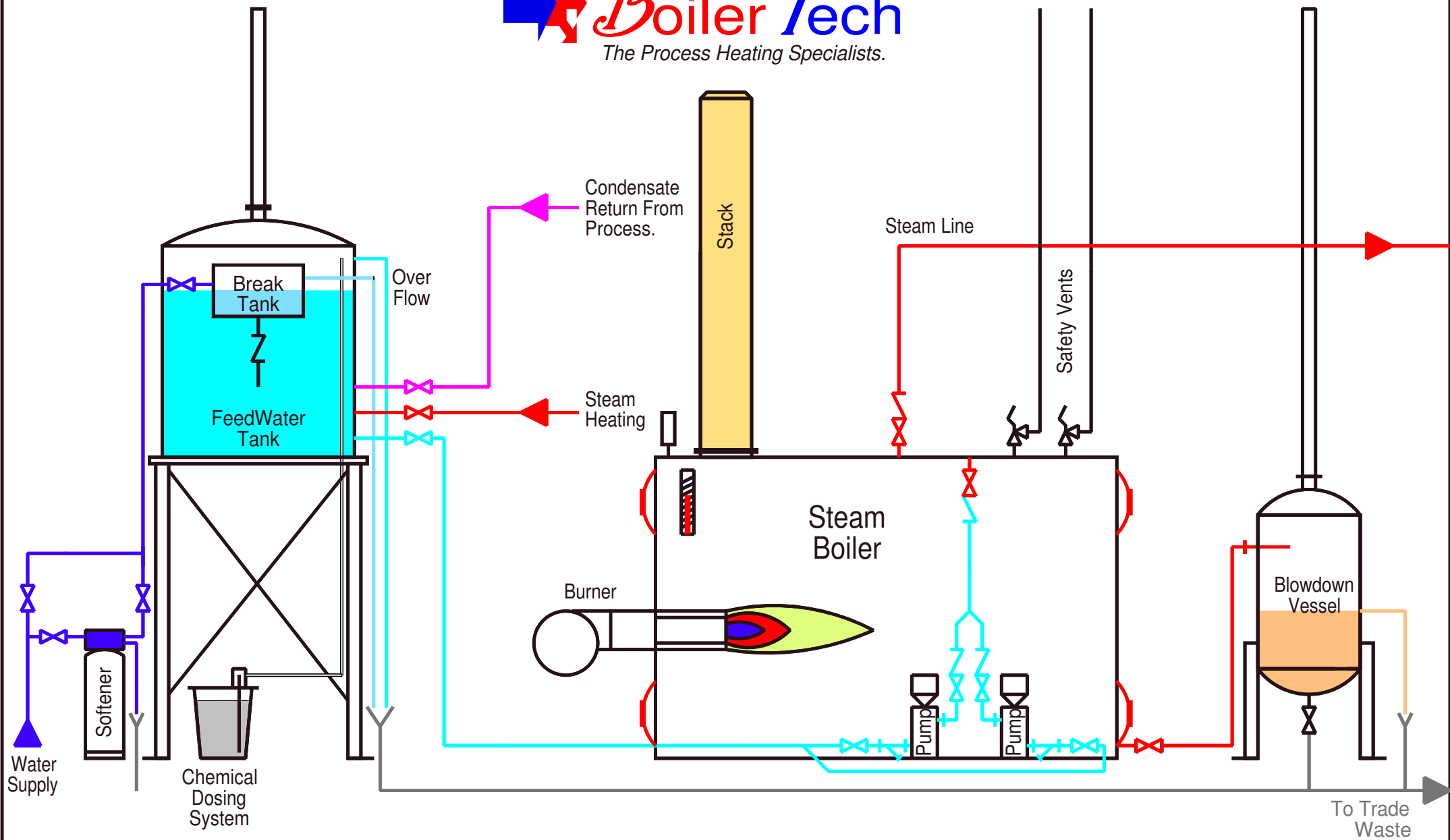
TYPICAL STEAM BOILER & ANCILLARY EQUIPMENT LAYOUT.
